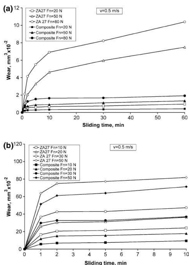
Fig. 1. Wear curves of tested materials; a) Lubricated sliding, b) Dry sliding [2,4].
