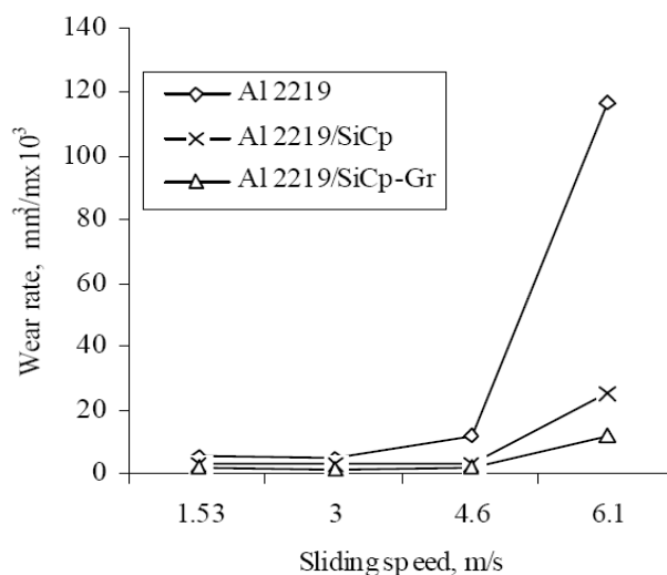
Fig. 8. The wear rate variation with sliding speed for both composites and its matrix alloy [20-22].
