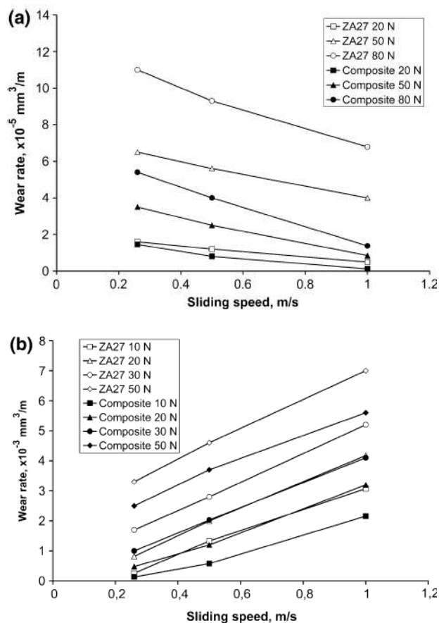
Fig. 3. Wear curves of tested materials; a) Lubricated sliding, b) Dry sliding [2, 4].
