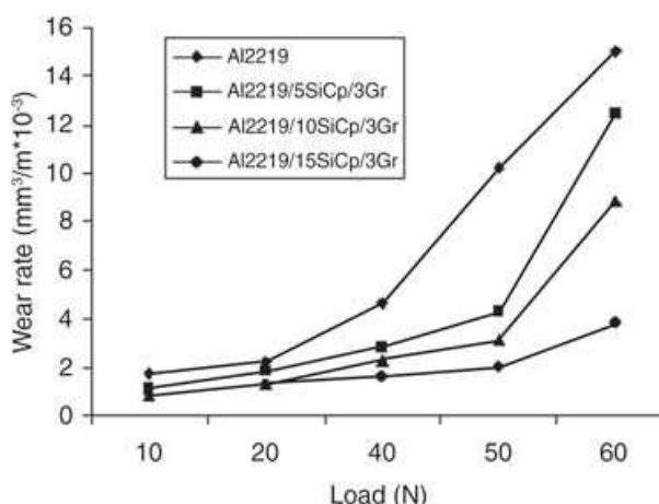
Fig. 9. Variation of wear rate with applied load at a sliding speed of 3 m/s for a sliding distance of 5000 m [20-22].
