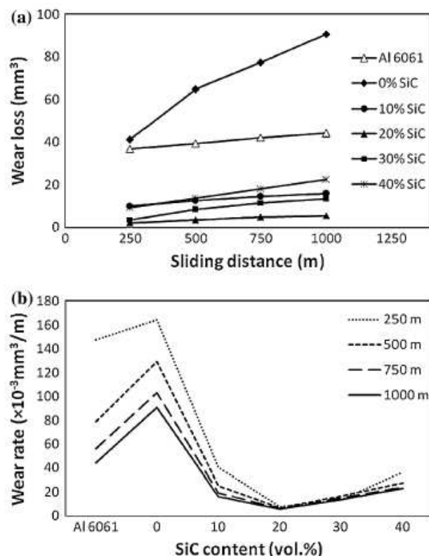
Fig. 13. The variation of a wear loss with a) sliding distance and b) wear rate with SiC content for the hybrid composites containing 9 vol.% Gr particles [31].
