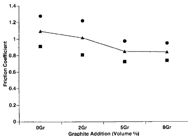
Fig. 6. Variations of friction coefficient with the percentage of graphite addition [19].
