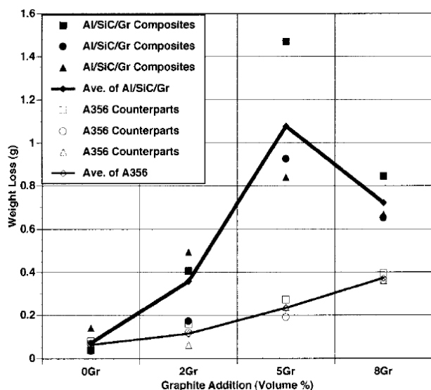
Fig. 7. Weight loss of the composites and the counterparts for various graphite additions [19].
