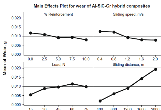
Fig. 10. Main effect plot of effect of factors on wear of Al-SiC-Gr hybrid composites [23-25].
