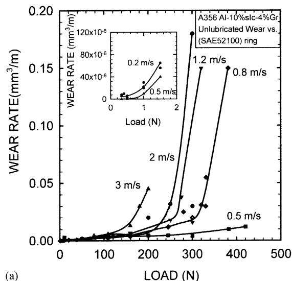
Fig. 11. Wear volume vs. applied load [26].
