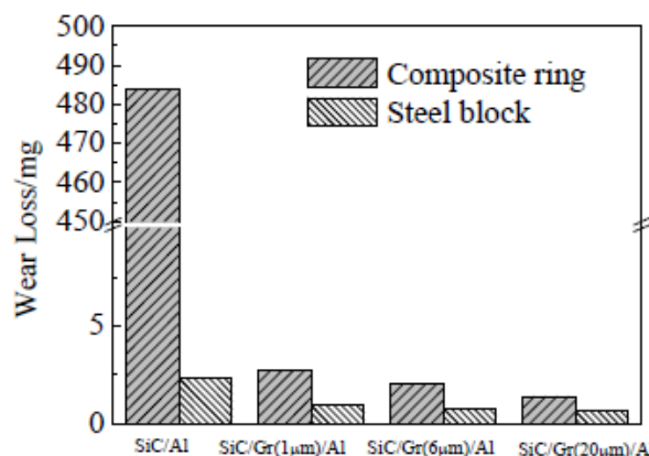
Fig. 12. Wear loss of the composites and counterfaces of wear process for SiC/Al and SiC/Gr/Al [27-29].
