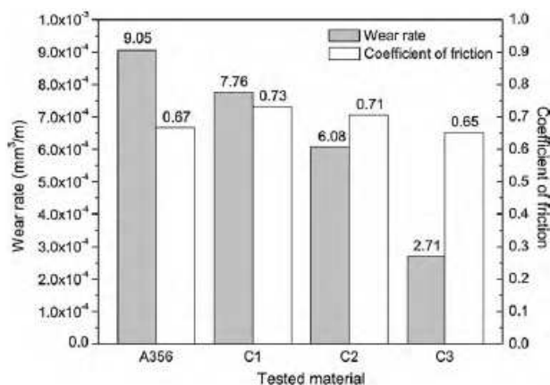
Fig. 14. Wear rate and coefficient of friction values of heat treated (T6) A356 aluminium alloy, composite C1 (with 10 wt% Al 2 O 3 particles), composite C2 (with 10 wt% SiC particles), and composite C3 (with 10 wt% SiC and 1 wt% graphite particles) [32,33].
