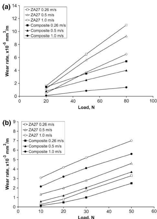
Fig. 2. Wear volume vs. applied load; a) Lubricated sliding, b) Dry sliding [2,4].
