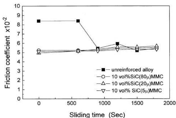
Fig. 4. Friction coefficient vs sliding time for unreinforced ZA27 alloy and MMCs containing SiC particles of various sizes [10].
