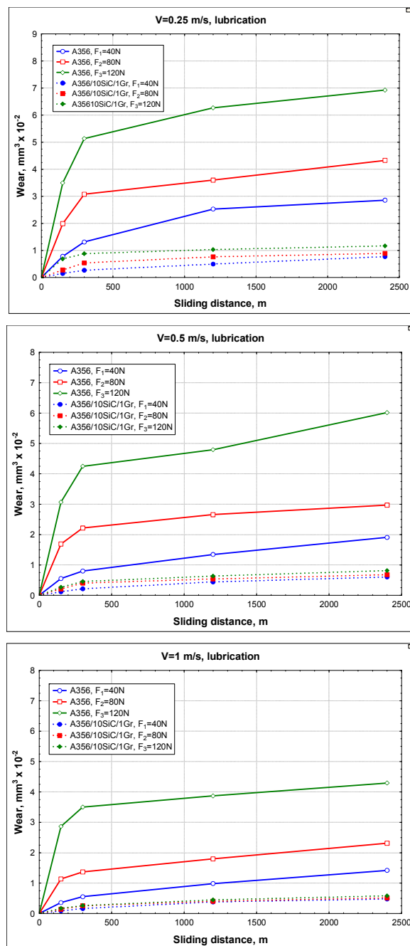
Fig. 4. Wear volume for all three values of sliding speed.
