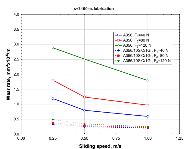
Fig. 5. Wear rate dependence on sliding speed.
