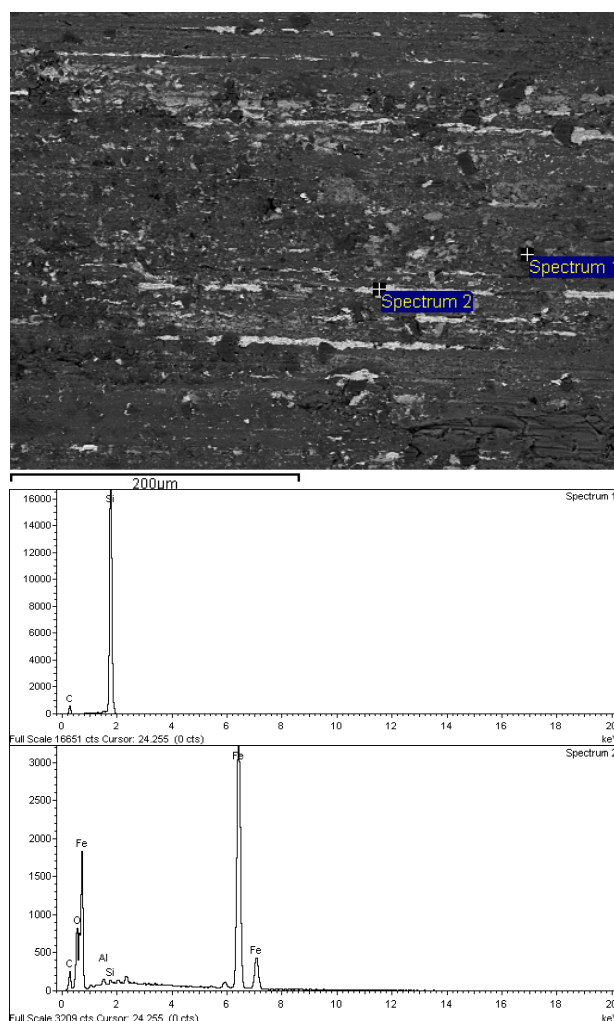
Fig. 12. EDS analysis A356/10SiC/1Gr, 120 N, 0.25 m/s, SEM.
