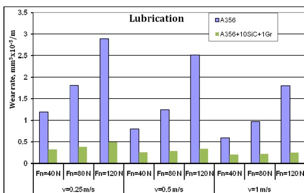
Fig. 7. Wear rate dependence on normal load and sliding speed.
