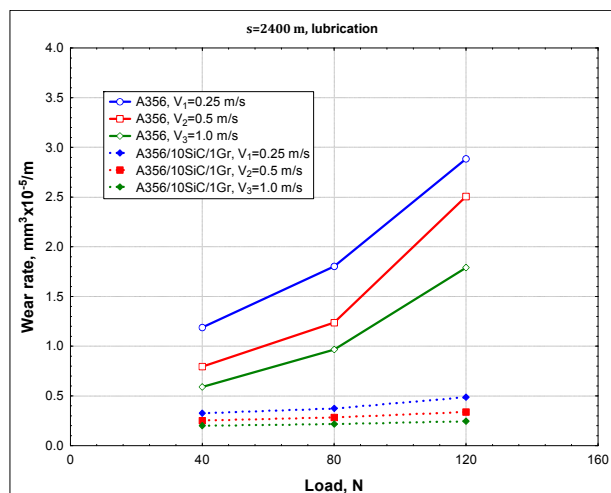
Fig. 6. Wear rate dependence on normal load.
