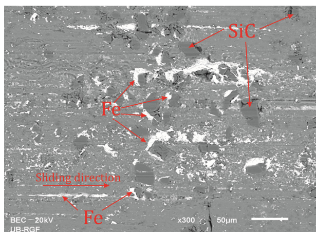
Fig. 11. The accumulation of iron in the composite A356/10SiC/1Gr, 120 N, 0.25 m/s.
