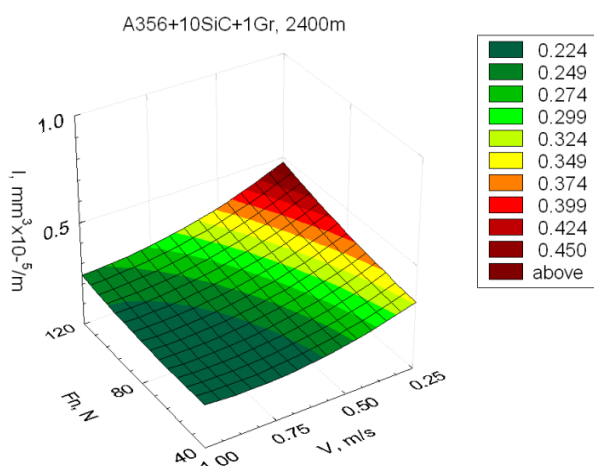
Fig. 10. Wear rate dependence on the hybrid composites A356/10SiC/1Gr.
