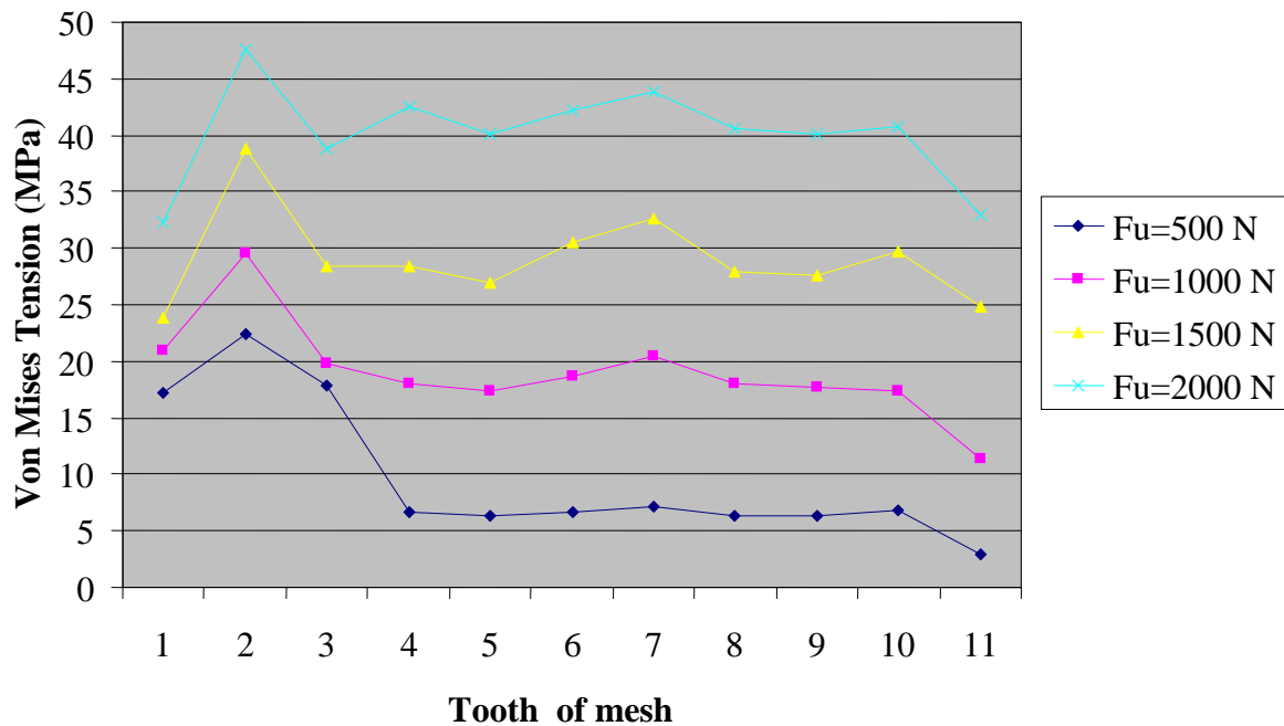
Figure 9. Load distribution on teeth in mesh due to the pre-tensioning force
