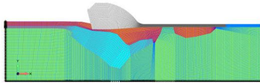
Figure 1. FE model of overflow dam section
