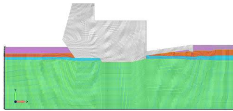
Figure 2. FE model of powerhouse dam section
