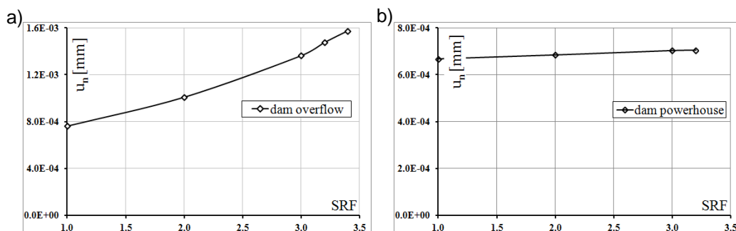
Figure 4. Maximal horizontal displacement of the dam in function of SRF
