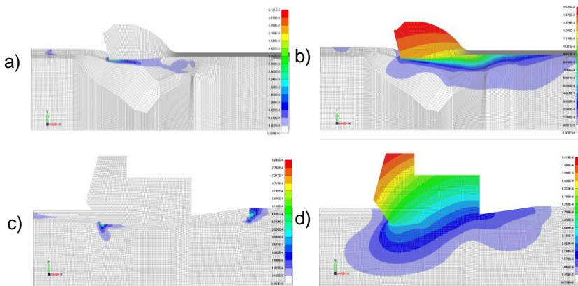
Figure 3. Plastic strain and total translation for maximal SSR factor
