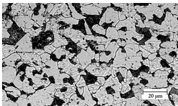
Fig.1. Typical microstructure of high strength steels [2]
