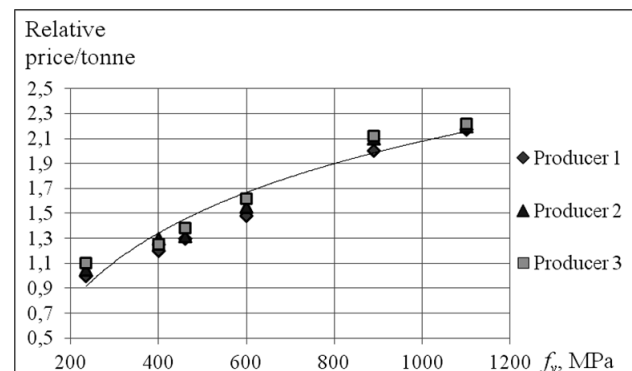
Fig.4. The average referent prices of high strength steels in function of yield limit
