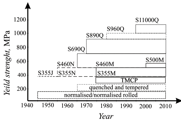
Fig.3. The development of general purpose constructional steels
