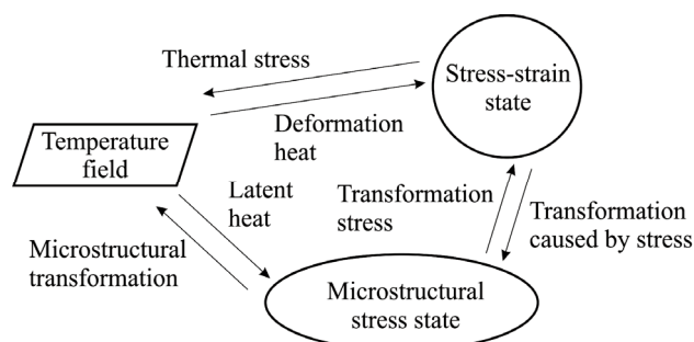
Fig.2. The influential factors to real stress state in exploitation
