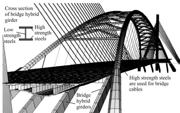
Fig.6. Bridge design with hybrid girders
