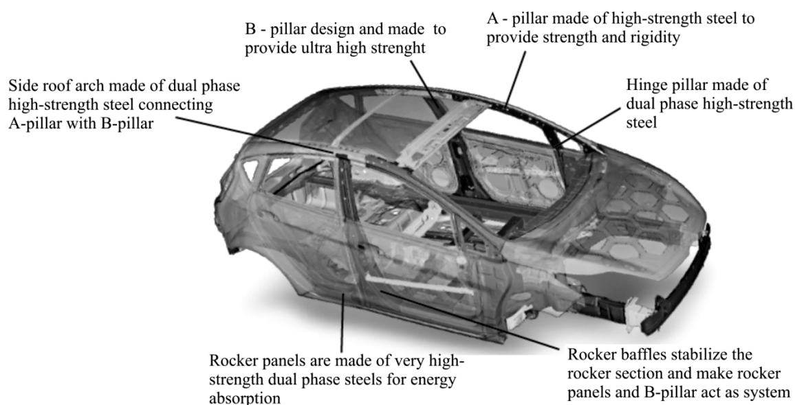
Fig. 2. Materials of specific zones of car body
